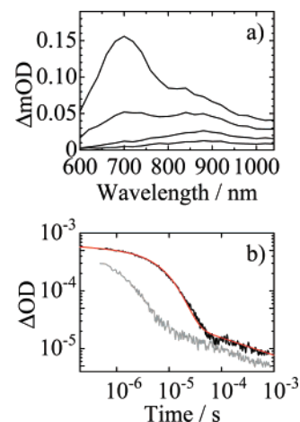
Figure 6. (a) Transient absorption spectra of the P(T 10 PhT 10 )/PCBM blend film at 10, 20, 100, and 800 \mu s after the laser excitation from top to bottom. (b) Transient absorption decays of the P(T 10 PhT 10 )/PCBM blend film monitored at 700 nm under Ar (black line) and O 2 (gray line) atmospheres at room temperature.
