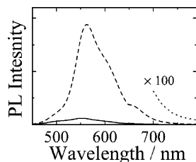
Figure 5. PL spectra of P(T 10 PhT 10 )/PCBM blend (solid line) and P(T 10 -PhT 10 ) pristine (broken line) films. The PL intensity was corrected for variation in the absorption at an excitation wavelength of 420 nm. The PL tail of P(T 10 PhT 10 )/PCBM blend film is multiplied by 100 (dotted line).
