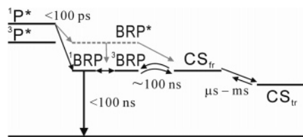
Scheme 2. Energy Diagram for Charge Formation via BRPs Proposed for the More Crystalline Polymer/PCBM Blend Films a
