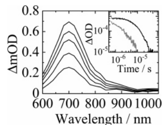
Figure 3. Transient absorption spectra of the P(T_{10}PhT_{10}) pristine film at 1, 2, 3, 5, and 8 \mu s after the laser excitation from top to bottom. (Inset) Transient absorption decays of the P(T_{10}PhT_{10}) pristine film monitored at 700 nm under Ar (black line) and O_2 (gray line) atmospheres at room temperature.
