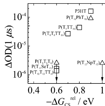
Figure 10. Transient absorbance at 1 \mu s of the blend films plotted against -\Delta G_{CS}^{rel} estimated as E_S - (IP - EA) where E_S is the energy level of polymer singlet excitons. The absorbance was corrected for variation in the absorption at the excitation wavelength and an extrapolated value at 1 \mu s estimated from the power-law decay at the longer time domain, measured at a probe wavelength of 1000 nm. The open triangles and squares represent data for the amorphous polymers and the more crystalline polymers, respectively. The arrows below data points indicate upper limit values. The low charge generation yield for P( T_{12}NpT_{12} ) is assigned to singlet energy transfer from P( T_{12}NpT_{12} ) to PCBM competing effectively with charge separation.
