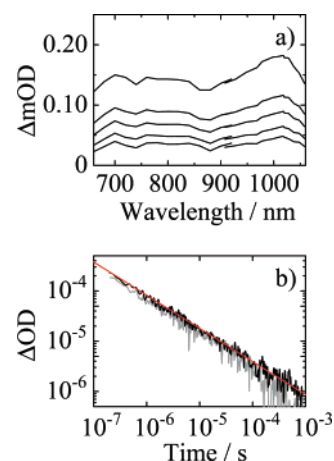
Figure 8. (a) Transient absorption spectra of the P3HT/PCBM blend film at 1, 2, 3, 5, and 8 \mu\text{s} after the laser excitation from top to bottom. (b) Transient absorption decays of the P3HT/PCBM blend film monitored at 1000 nm under Ar (black line) and O 2 (gray line) atmospheres at room temperature.
