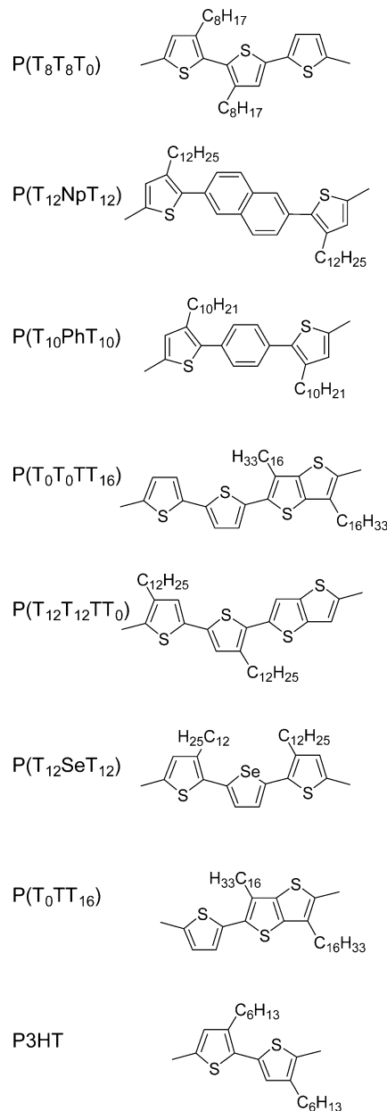
Chart 1. Chemical Structures of Various Polythiophenes with Different IP: from the Top: P(T 8 T 8 T 0 ), P(T 12 NpT 12 ), P(T 10 PhT 10 ), P(T 0 T 0 TT 16 ), P(T 12 T 12 TT 0 ), P(T 12 SeT 12 ), P(T 0 TT 16 ), P3HT
