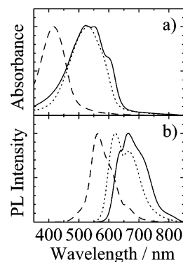
Figure 1. Absorption and PL spectra of P3HT (—), P(T 0 T 0 TT 16 ) (···), and P(T 10 PhT 10 ) (---) pristine films at room temperature.
