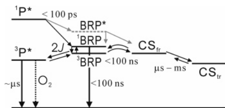
Scheme 1. Energy Diagram for Charge Formation via BRPs Proposed for the Amorphous Polymer/PCBM Blend Films a
