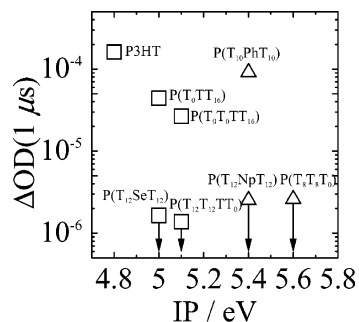
Figure 9. Transient absorbance at 1 \mu\text{s} of the blend films plotted against polymer IPs. The absorbance was corrected for variation in the absorption at the excitation wavelength and an extrapolated value at 1 \mu\text{s} estimated from the power-law decay at the longer time domain, measured at a probe wavelength of 1000 nm. The open triangles and squares represent data for the amorphous polymers and the more crystalline polymers, respectively. The arrows below data points indicate upper limit values.
