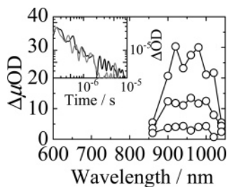
Figure 4. Transient absorption spectra of the P(T 0 T 0 TT 16 ) pristine film at 0.3, 0.5, and 1 \mu s after the laser excitation from top to bottom. (Inset) Transient absorption decays of the P(T 0 T 0 TT 16 ) pristine film monitored at 960 nm under Ar (black line) and O 2 (gray line) atmospheres at room temperature.
