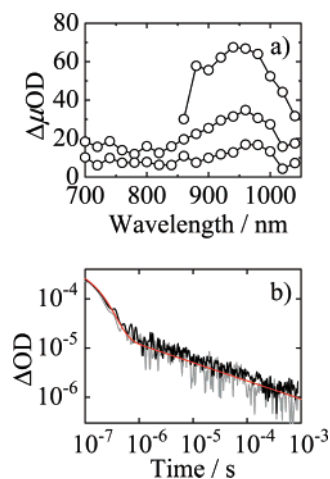
Figure 7. (a) Transient absorption spectra of the P(T 0 T 0 TT 16 )/PCBM blend film at 0.3, 0.5, and 1 \mu\text{s} after the laser excitation from top to bottom. (b) Transient absorption decays of the P(T 0 T 0 TT 16 )/PCBM blend film monitored at 960 nm under Ar (black line) and O 2 (gray line) atmospheres at room temperature.
