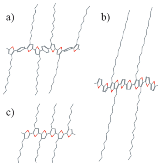
Figure 2. Minimum-energy molecular structures calculated by the MOPAC program: (a) 3-mer of P(T_{10}PhT_{10}) , (b) 2.5-mer of P(T_0T_0TT_{16}) , (c) 6-mer of P3HT.
